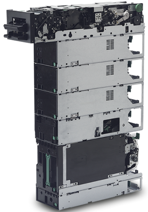
Recycling configuration of GSR50
